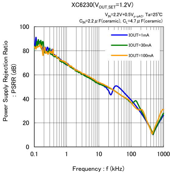
(16) Power Supply Rejection Ratio
