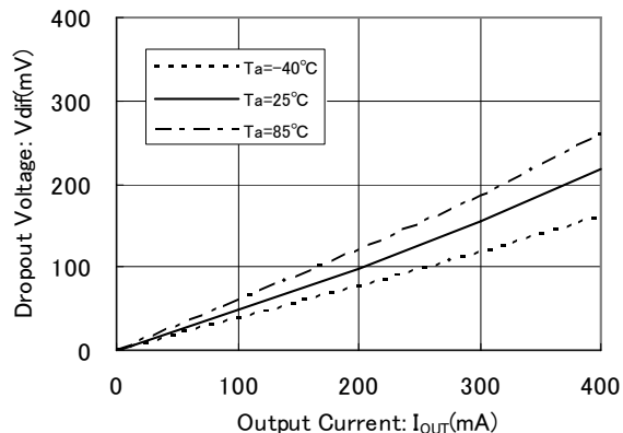
XC6601B121MR ( V_{gs}^{(*1)}=2.1\text{V} )
