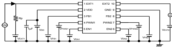
Circuit
