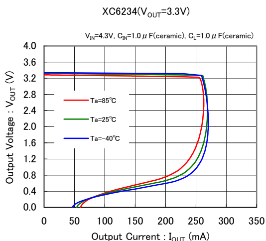
(1) Output Voltage vs. Output Current (Continued)
