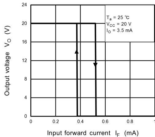
Fig. 12.2.4 V_O - I_F (HYS)
