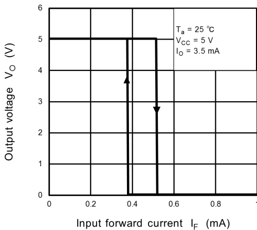
Fig. 12.2.3 V_O - I_F (HYS)
