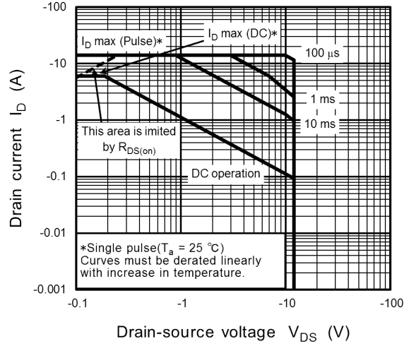
Fig. 7.14 Safe Operating Area
