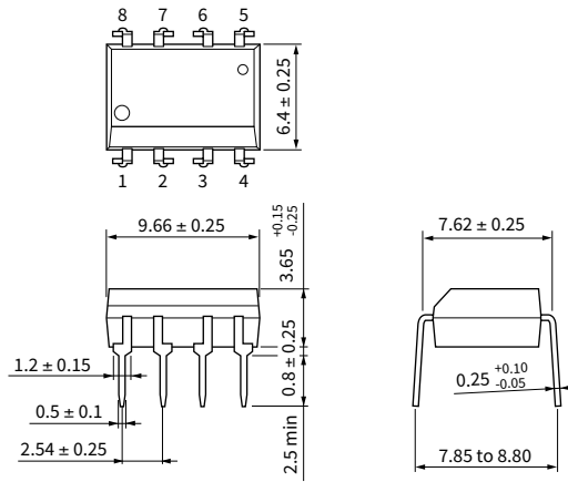
DIP8 (LF1)
