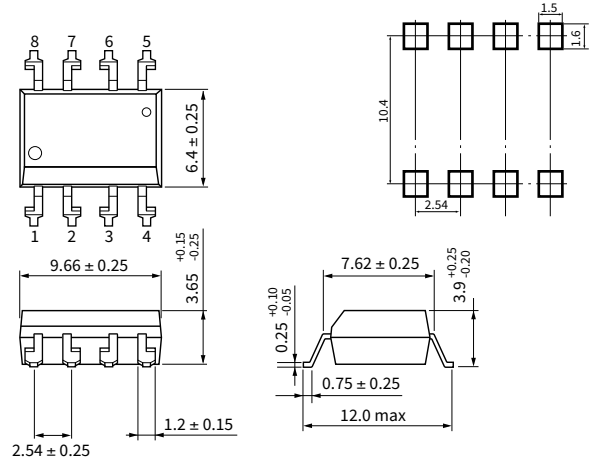
DIP8 (LF4)
