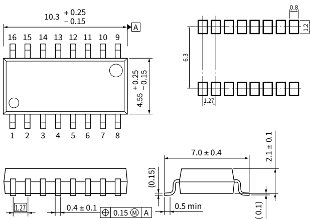
SO16
