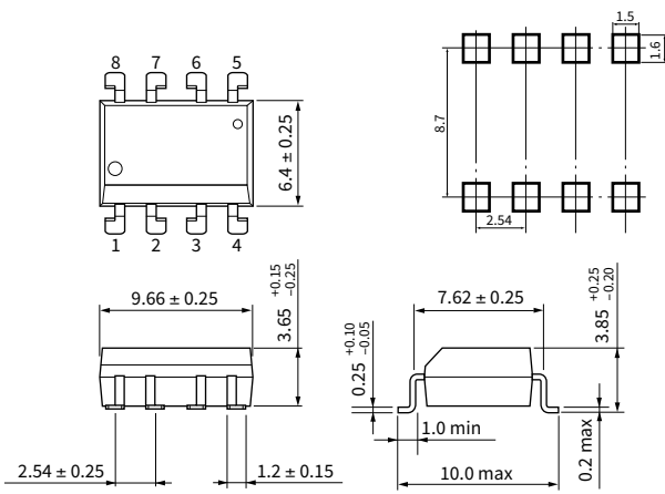
DIP8 (LF5)
