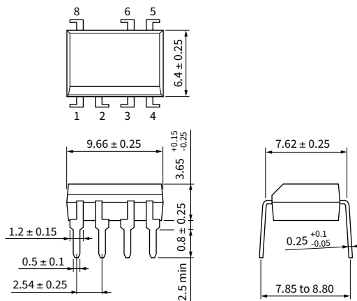
7 pin DIP8
