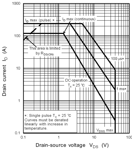
Fig. 8.14 Safe Operating Area (Guaranteed Maximum)
