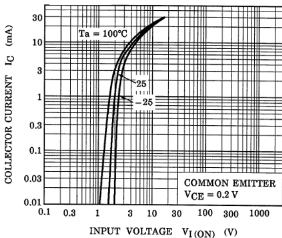
Fig. 10.3 RN1909 I_C - V_{I(ON)}
