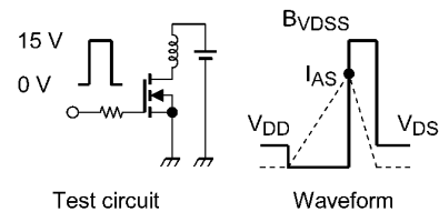
Fig. 9.15 Test Circuit/Waveform
