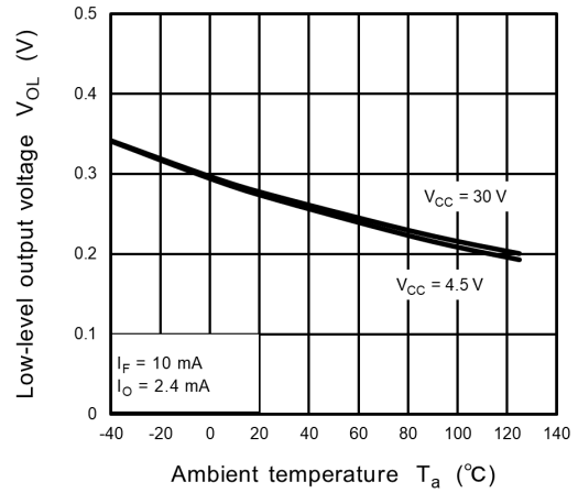
Fig. 12.2.8 V_{OL} - T_a
