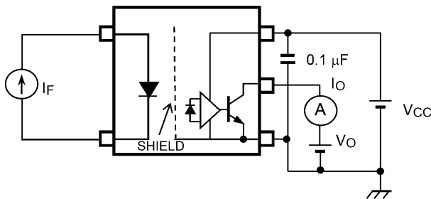
Fig. 12.1.5 I_O Test Circuit
