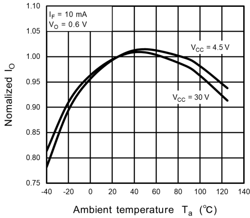
Fig. 12.2.7 I_O - T_a
