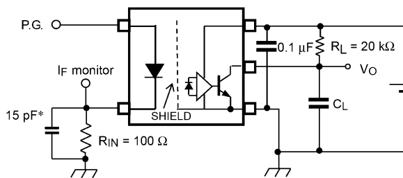
Fig. 12.1.6 Switching Time Test Circuit and Waveform
