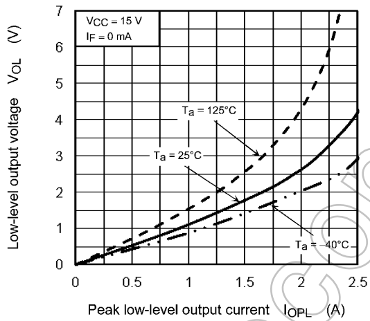
Fig. 12.2.9 V_{OL} - I_{OLP}
