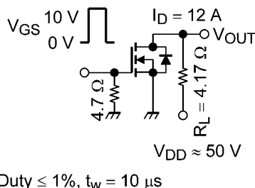
Duty \leq 1\% , t_w = 10\ \mu\text{s} Fig. 6.2.1 Switching Time Test Circuit
