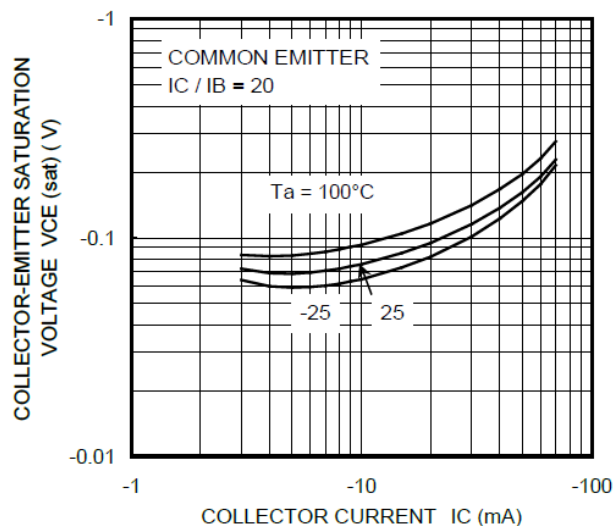
Fig. 10.20 RN2318 V_{CE(sat)}-I_C
