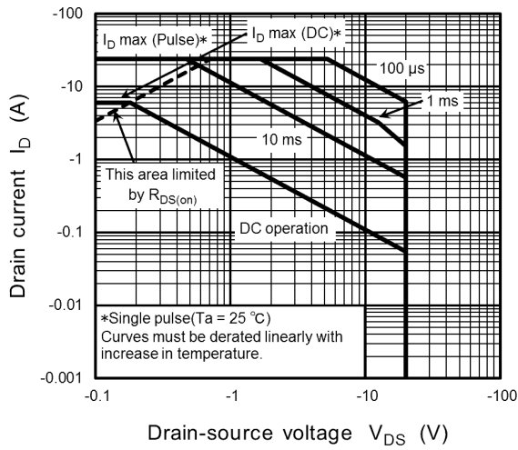
Fig. 7.15 Safe Operating Area
