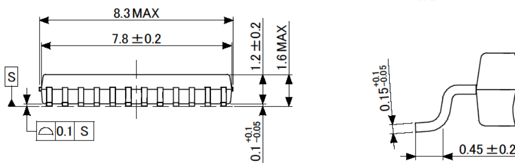
Figure 12.1 Package Dimensions
