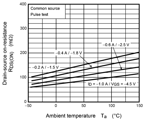
Fig. 8.5 R_{DS(ON)} - T_a
