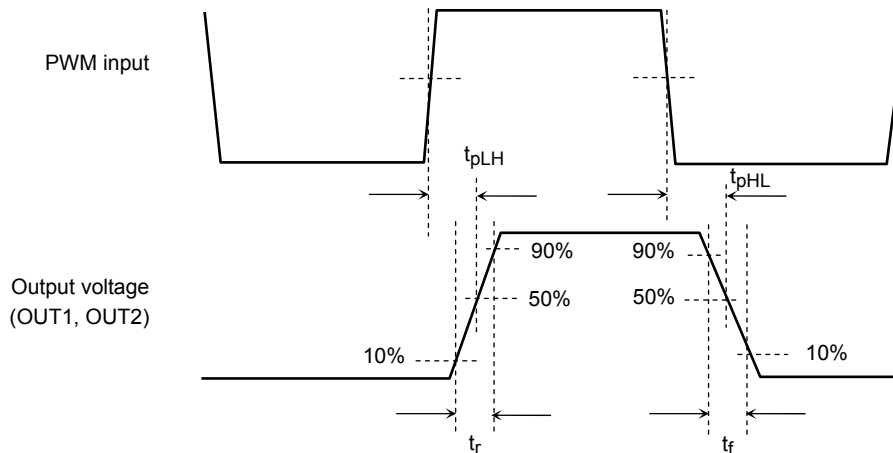
Switching Characteristics
