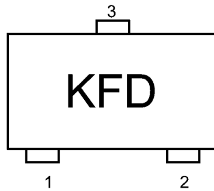
Fig. 6.1 Marking
