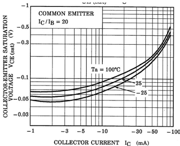
Fig. 10.23 RN2105 V_{CE(sat)}-I_C
