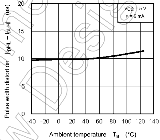
Fig. 12.2.10 |t_{pHL} - t_{pLH}| - T_a
