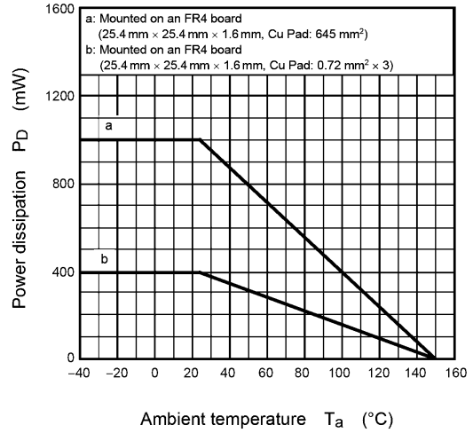
Fig. 8.14 P_D - T_a
