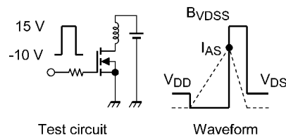
Fig. 9.15 Test Circuit/Waveform
