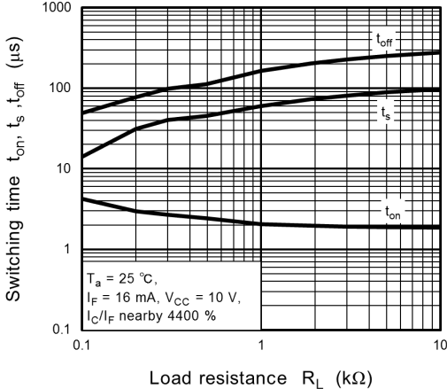
Fig. 11.13 Switching Time - R_L
