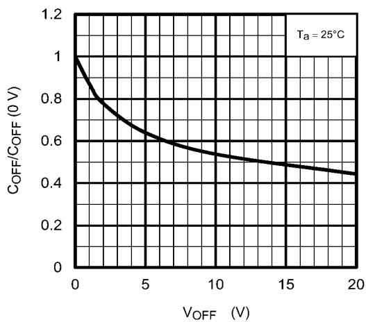
Fig. 12.11 C_{OFF}/C_{OFF}(0V) - V_{OFF}
