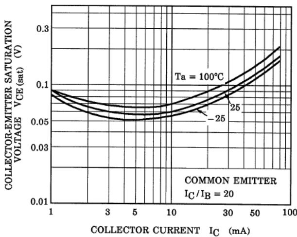
Fig. 10.21 RN1403 V_{CE(sat)}-I_C
