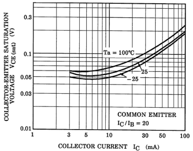
Fig. 10.20 RN1402 V_{CE(sat)}-I_C
