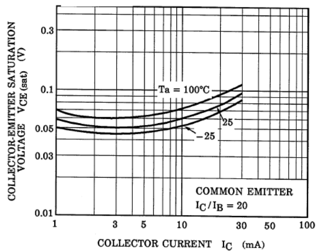
Fig. 10.22 RN1404 V_{CE(sat)}-I_C
