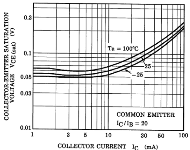
Fig. 10.24 RN1406 V_{CE(sat)}-I_C
