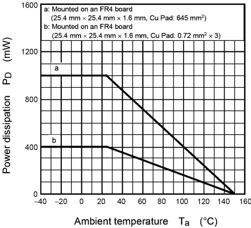
Fig. 8.13 P_D - T_a
