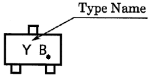
Fig. 10.2 Marking RN2102MFV
