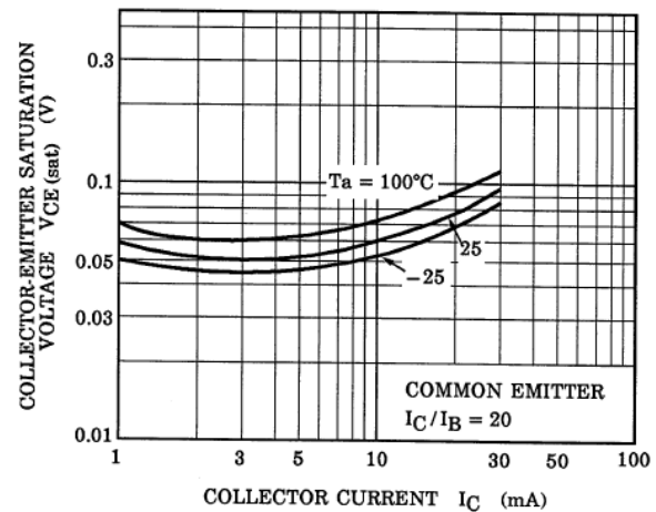
Fig. 10.22 RN1104 V_{CE(sat)}-I_C
