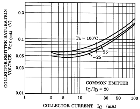
Fig. 10.20 RN1102 V_{CE(sat)}-I_C
