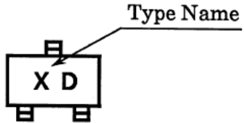
Fig. 9.4 Marking RN1104
