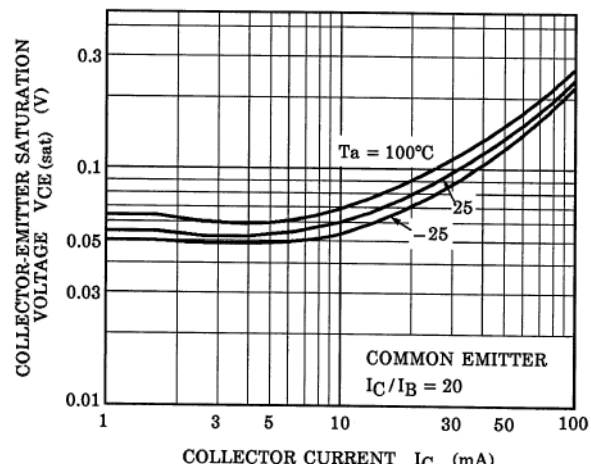
Fig. 10.24 RN1106 V_{CE(sat)}-I_C
