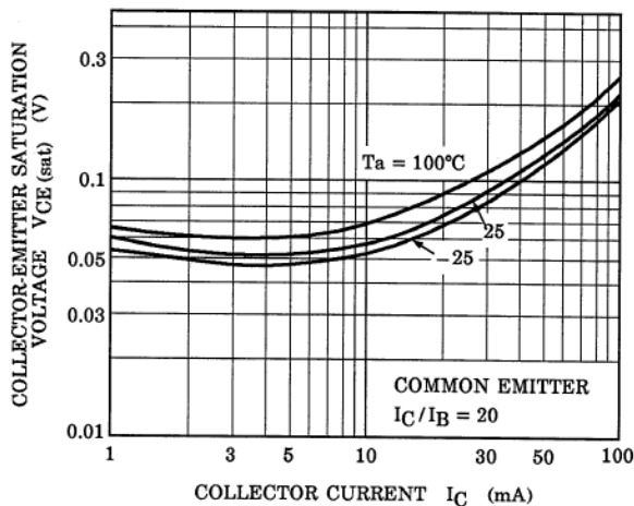
Fig. 10.23 RN1105 V_{CE(sat)}-I_C
