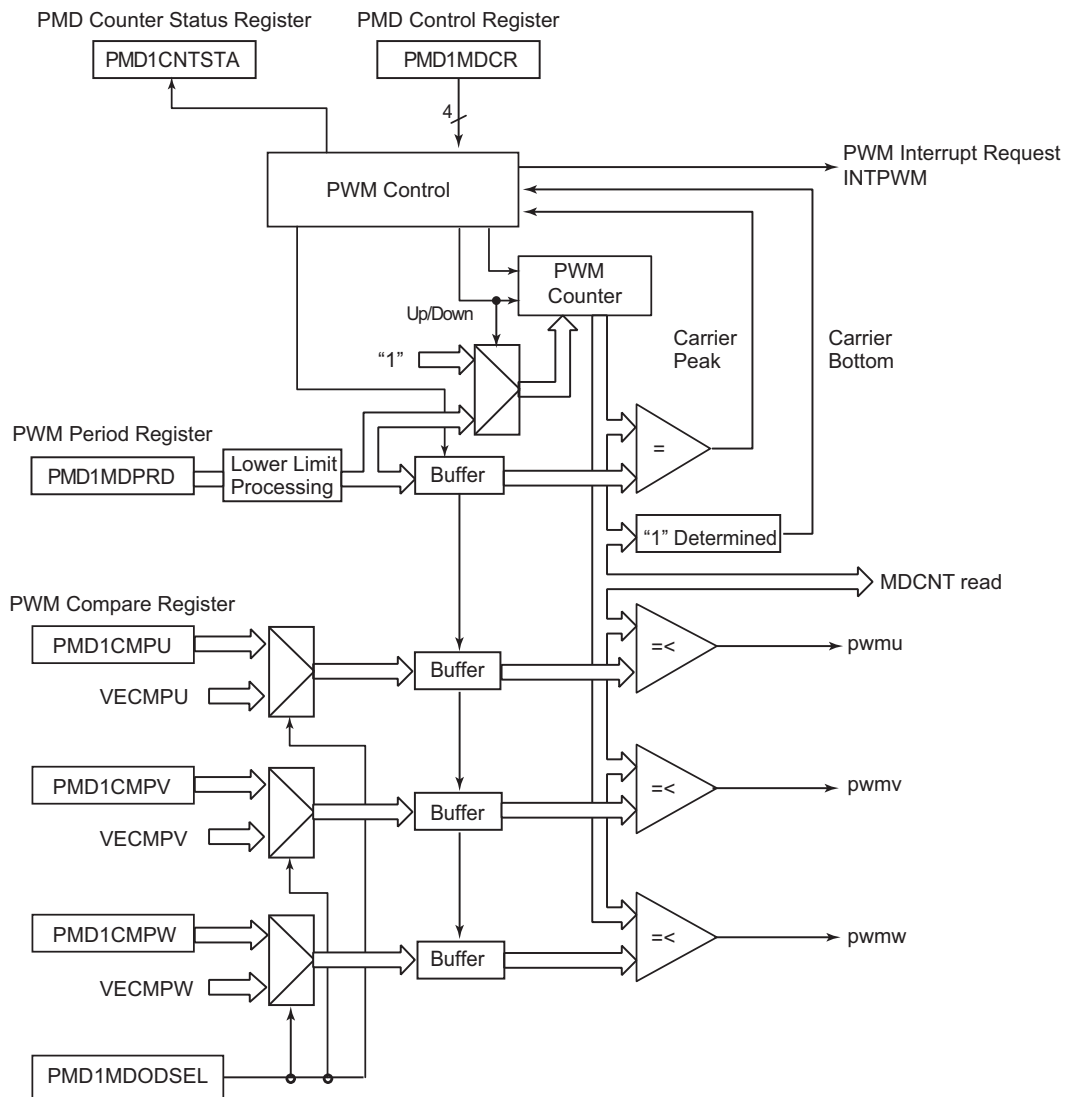
Figure 11-3 Pulse Width Modulation Circuit
