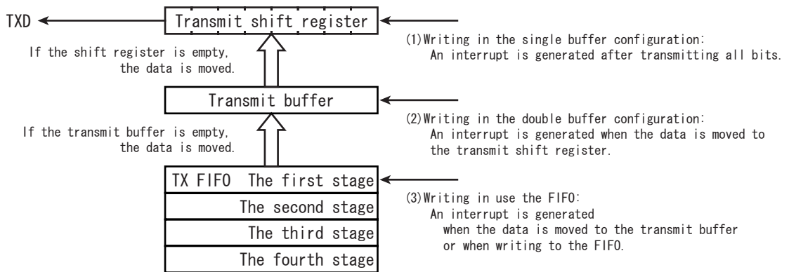
Figure 9-11 Transmit Buffer/FIFO Configuration Diagram
