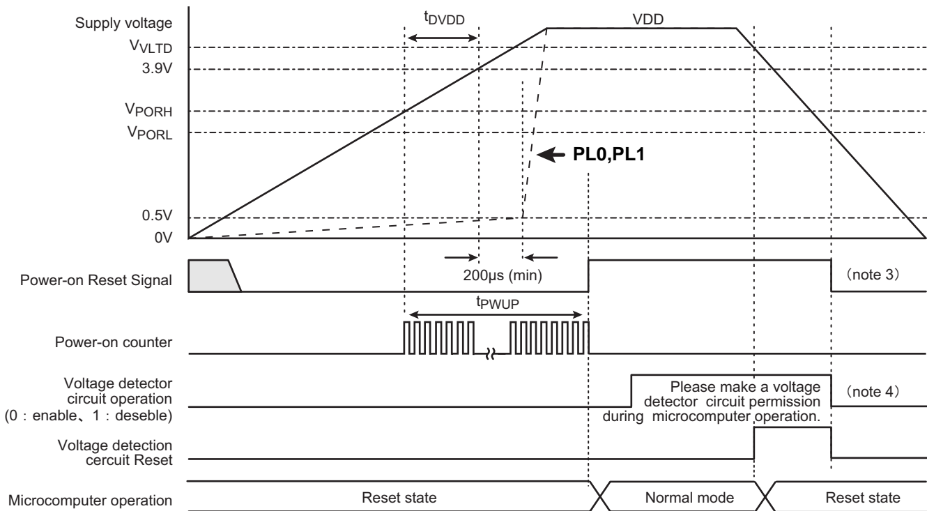
Figure 22-5 Powe on Sequence (Using Power On Reset only)
