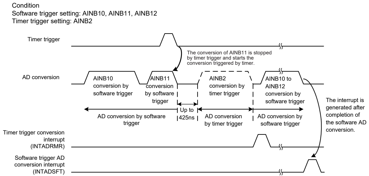
Figure 10-8 AD conversion by timer trigger
