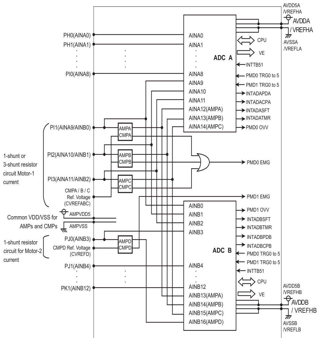
Figure 10-1 AD converters Block Diagram
