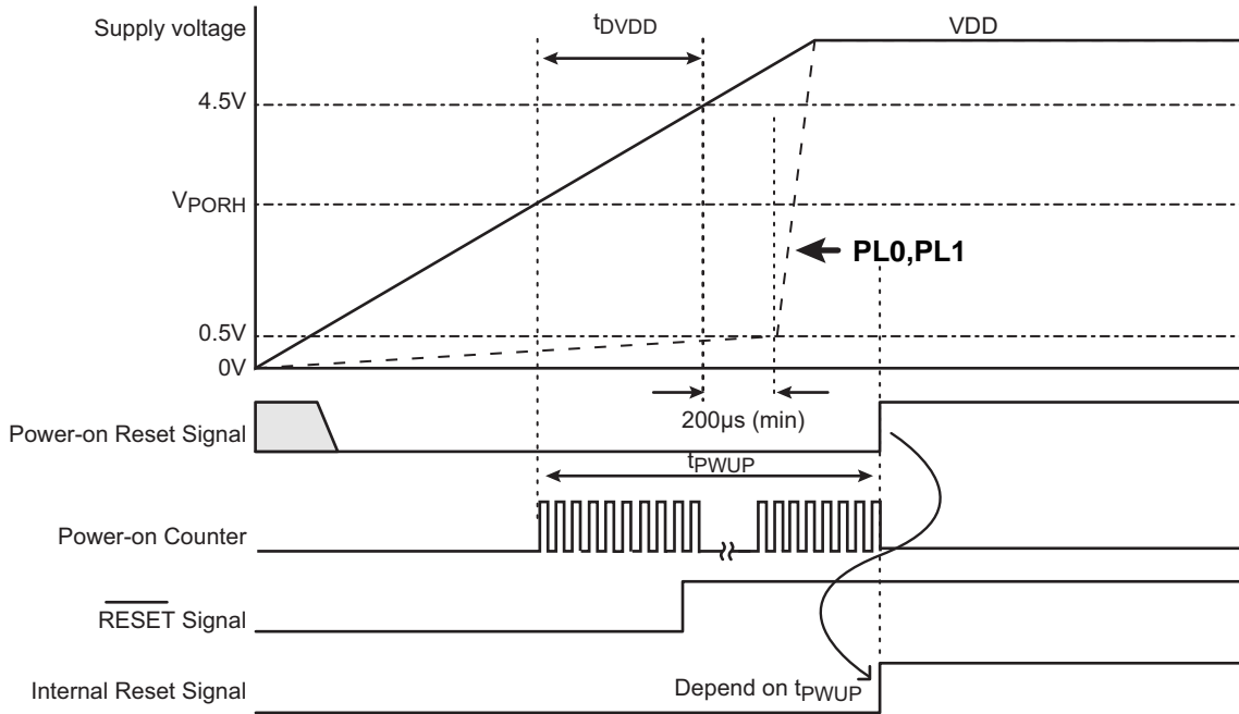
Figure 22-6 Power on Sequence ( Using POR and External reset ) (1)
