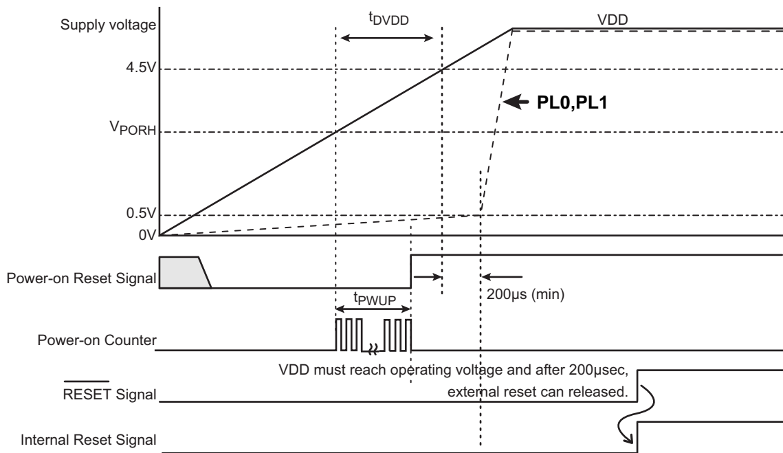
Figure 22-8 Power on Sequence ( t_{DVDD} > t_{PWUP} )
