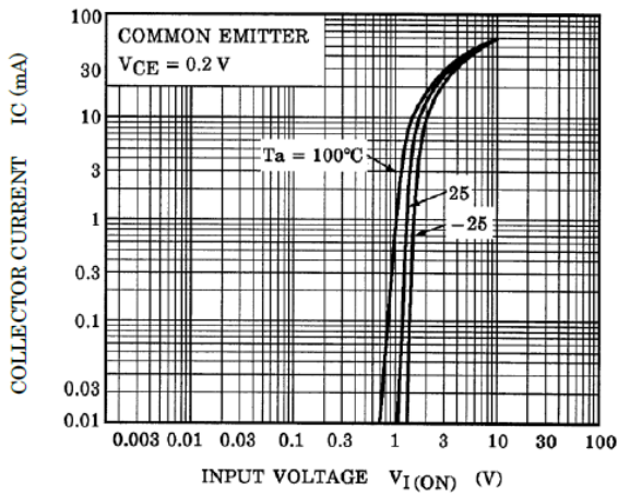
Fig. 10.1 RN1301 I_C - V_{I(ON)}
