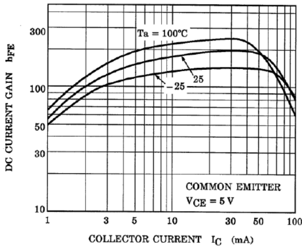
Fig. 10.17 RN1305 h_{FE}(\text{sat})-I_C
