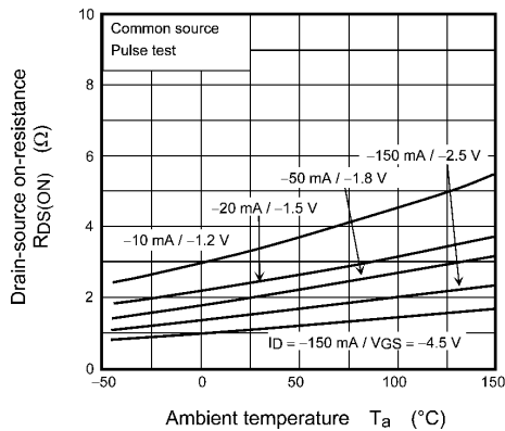
Fig. 7.5 R_{DS(ON)} - T_a
