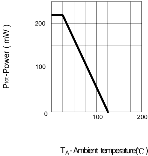
FIG.1- ADMISSIBLE POWER DISSIPATION VS. AMBIENT TEMPERATURE
