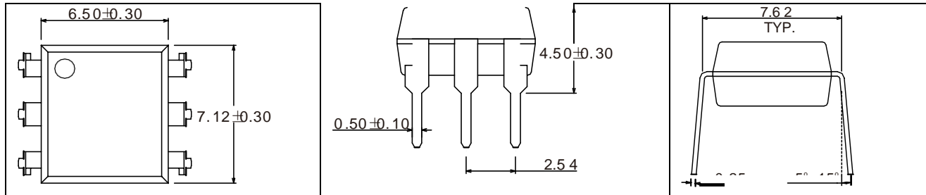
6 pin DIP
