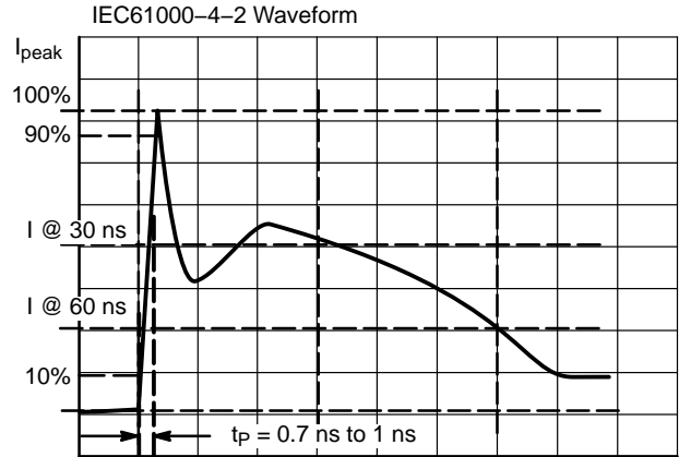
Figure 7. IEC61000-4-2 Spec
