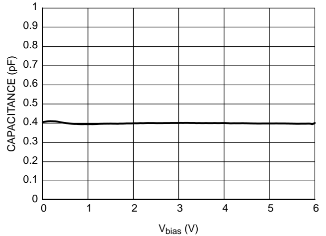
Figure 2. CV Characteristics
