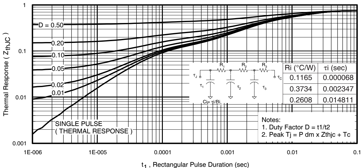
Fig 11. Maximum Effective Transient Thermal Immedance, Junction-to-Case
