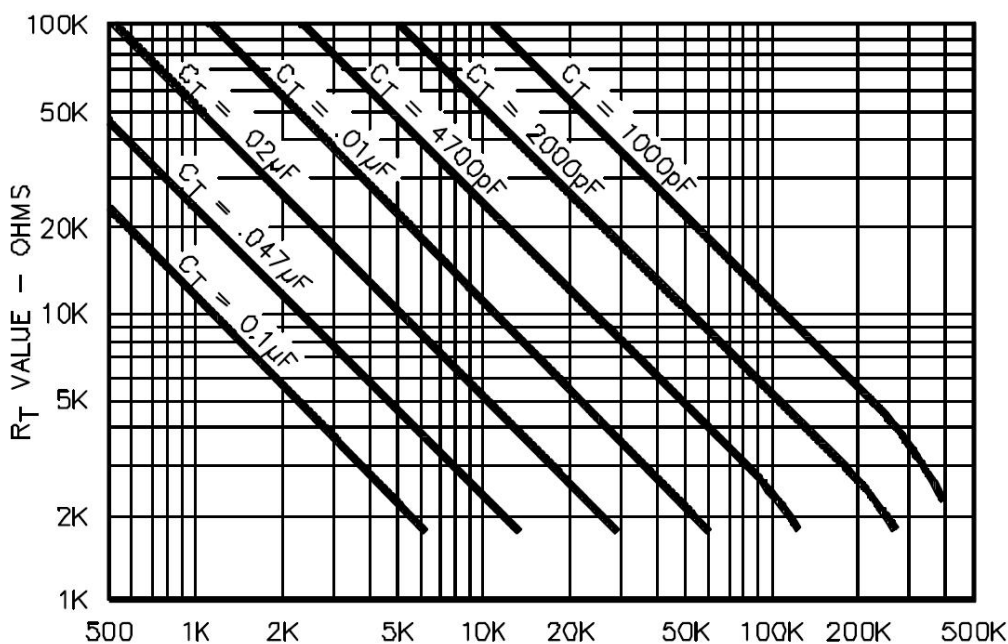
Relation between oscillation frequency and Rt, Ct
