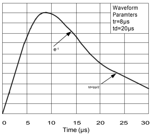
Figure3: Pulse Waveform
