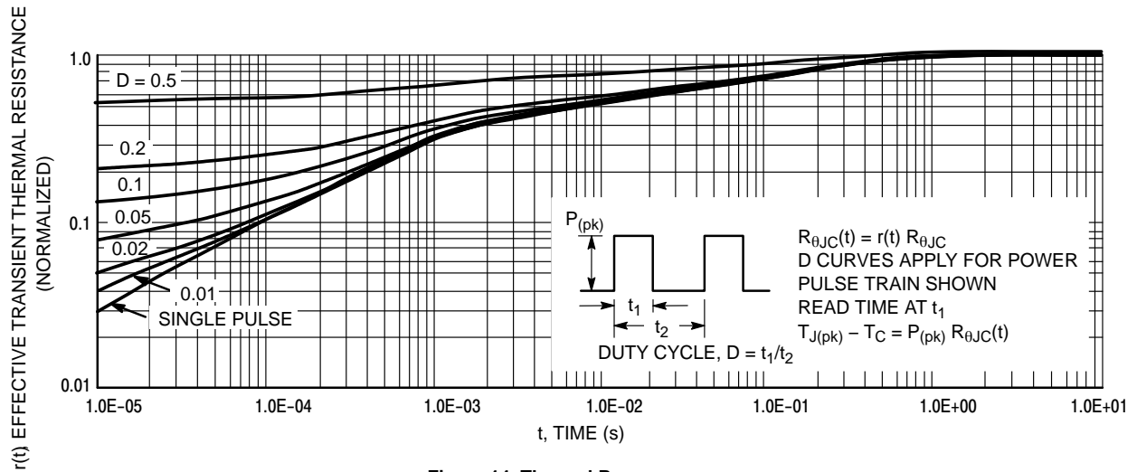
Figure 14. Thermal Response
