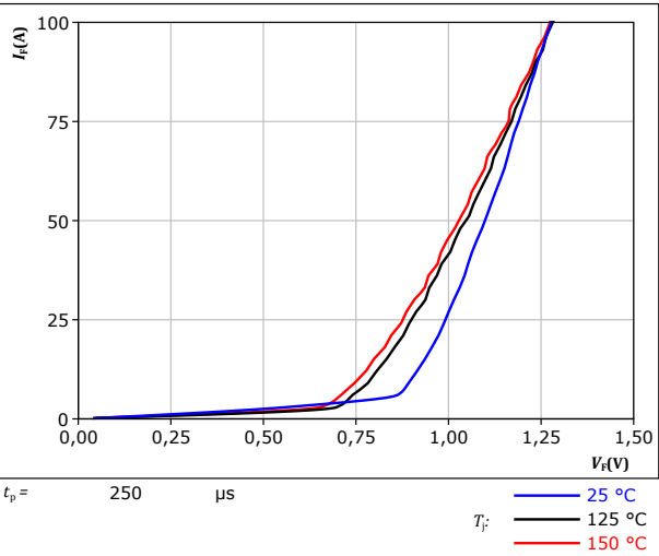
figure 9. Rectifier
