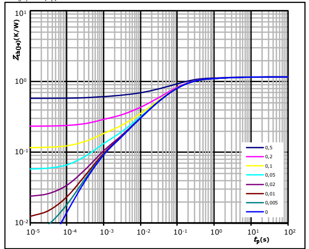
figure 4. IGBT
