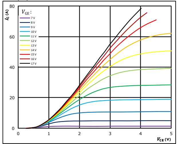
figure 2. IGBT
