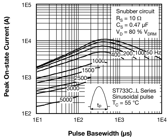
Fig. 13 - Frequency Characteristics
