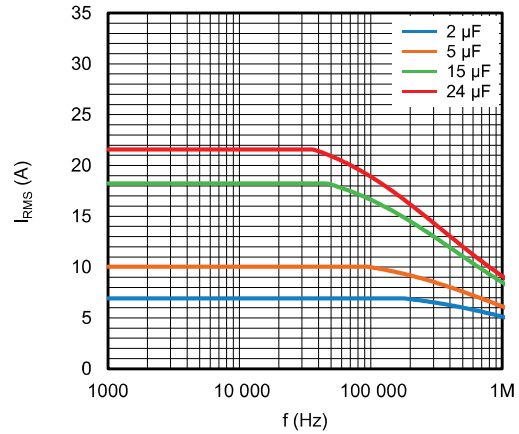
Maximum I_{RMS} vs. frequency for 1200 V, ambient temperature of 85 °C (typical curve)
