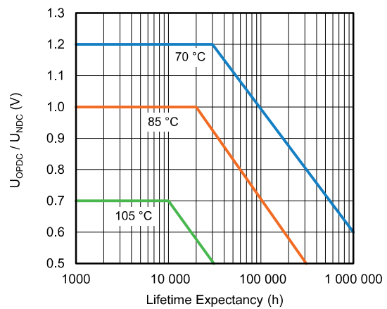
Lifetime expectancy by case temperature
