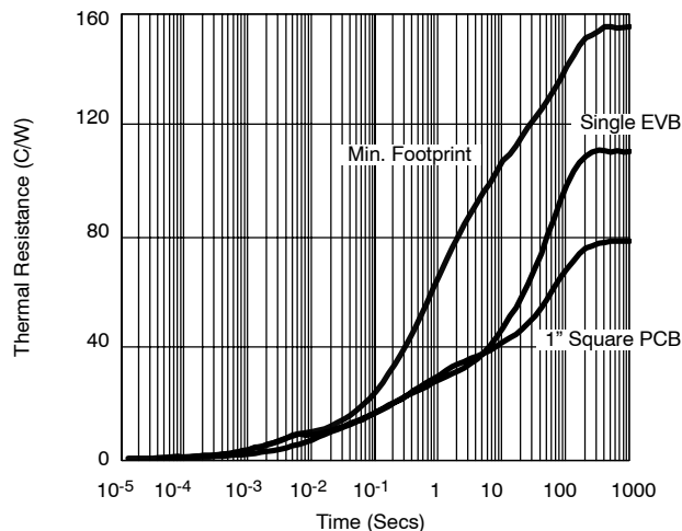
FIGURE 4. Single 1206-8 ChipFET
