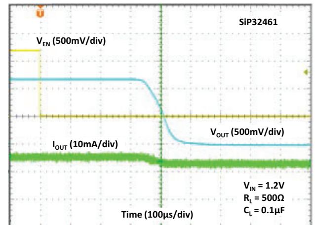
Fig. 37 - Turn-off Time
