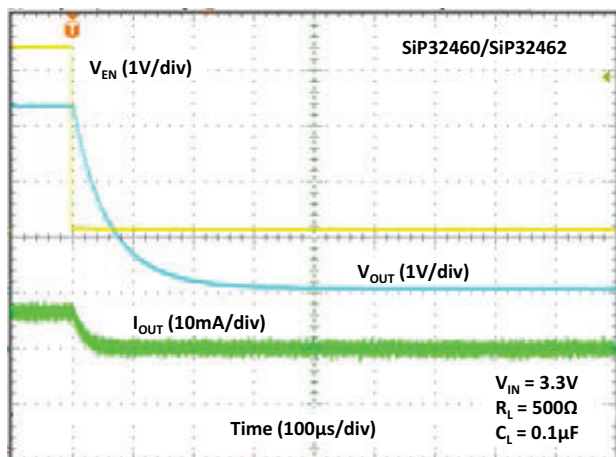
Fig. 34 - Turn-off Time
