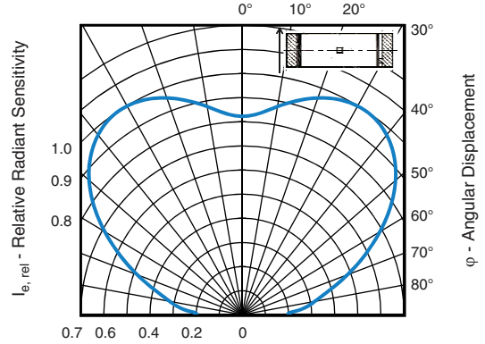
Fig. 7 - Relative Radiant Sensitivity vs. Angular Displacement - Vertical
