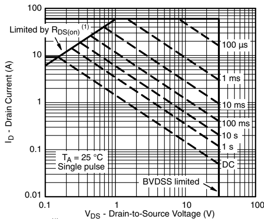
Safe Operating Area, Junction-to-Ambient ( 1 ) V_{GS} > minimum V_{GS} at which R_{DS(on)} is specified
