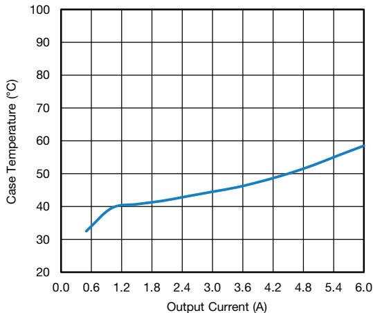
Fig. 19 - SiC462 Load Current vs. Case Temperature, VIN = 48 V, VOUT = 5 V
