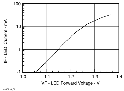
Fig. 4 - LED Forward Current vs. Forward Voltage
