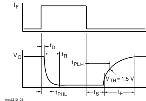
Fig. 2 - Switching Waveform
