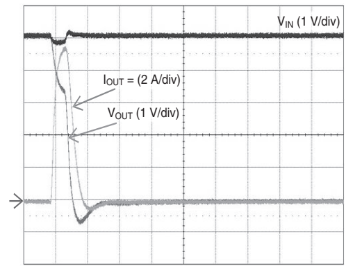
1 μs/div Short Circuit through 0.3 Ω, V in = 5 V
