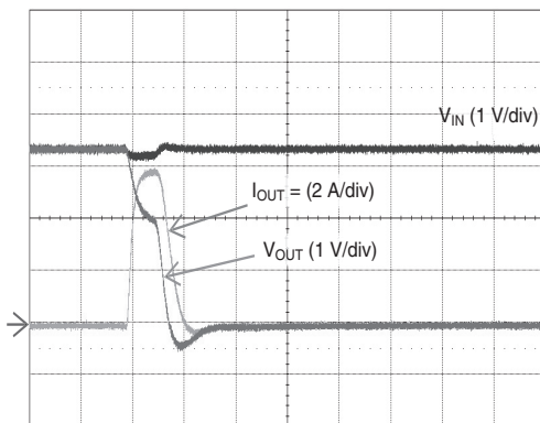
1 μs/div Short Circuit through 0.3 Ω, V in = 3.3 V
